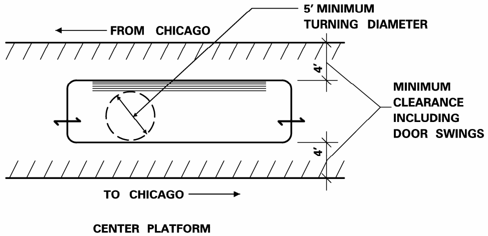
FIGURE III - 13 WARMING HOUSE SAMPLE LAYOUTS
