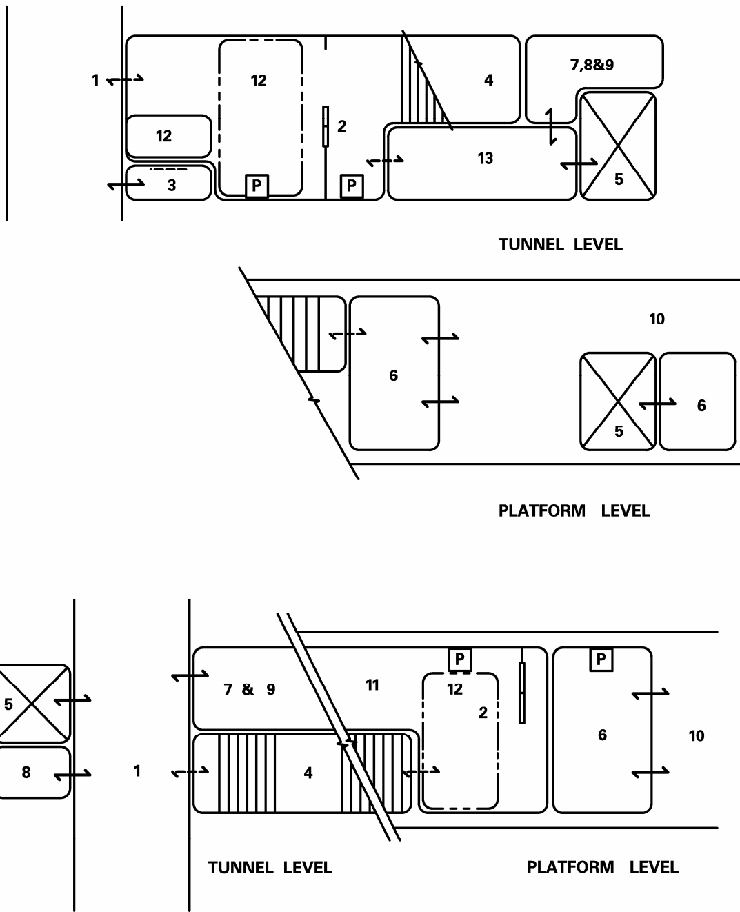
FIGURE III - 17 SAMPLE ELECTRIC TICKETHOUSE/HEADHOUSE LAYOUT AT A PED. TUNNEL CONT'
